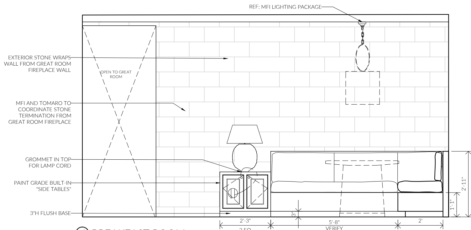
④ BREAKFAST ROOM
