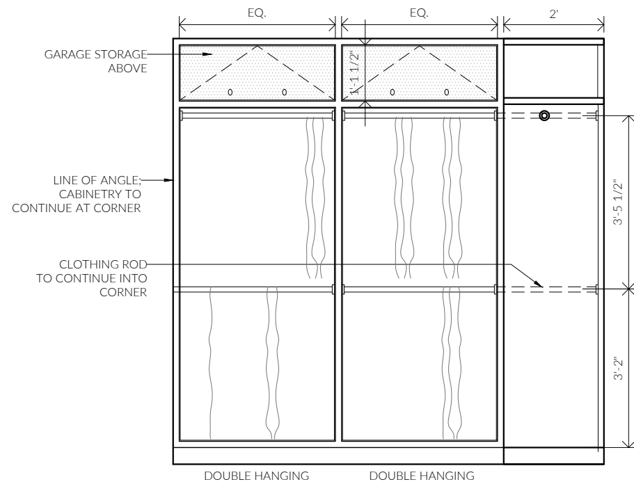
④ HER CLOSET
