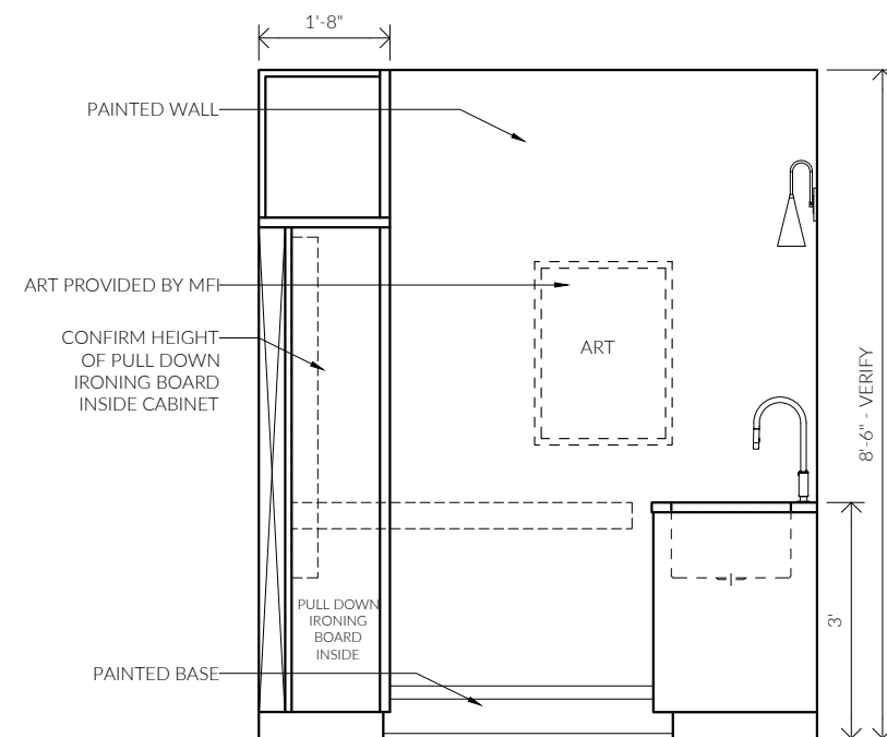
① LAUNDRY ROOM
