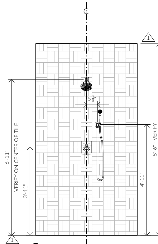
③ BATH 4 SHOWER
