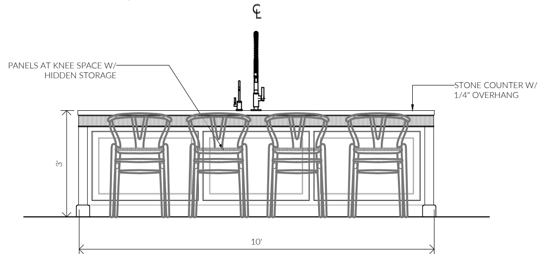
⑤ KITCHEN ISLAND SCALE: 3/8" = 1'0"
