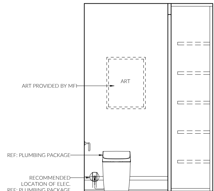
④ MASTER BATH W.C.
