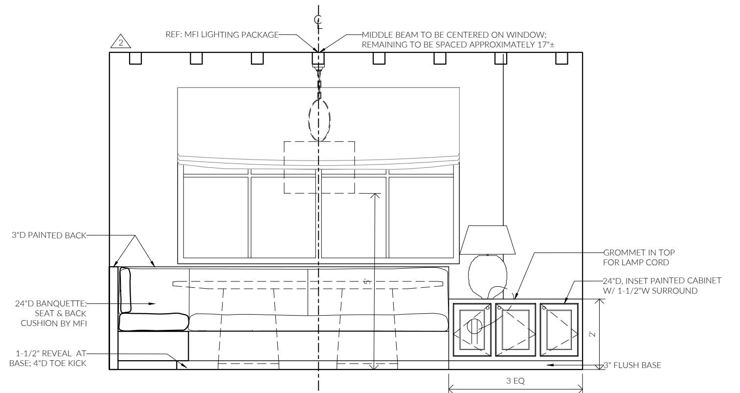
③ BREAKFAST ROOM
