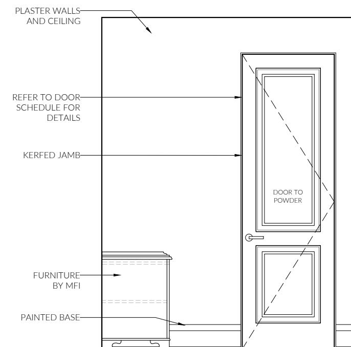
③ POWDER ROOM 02 VEST.
