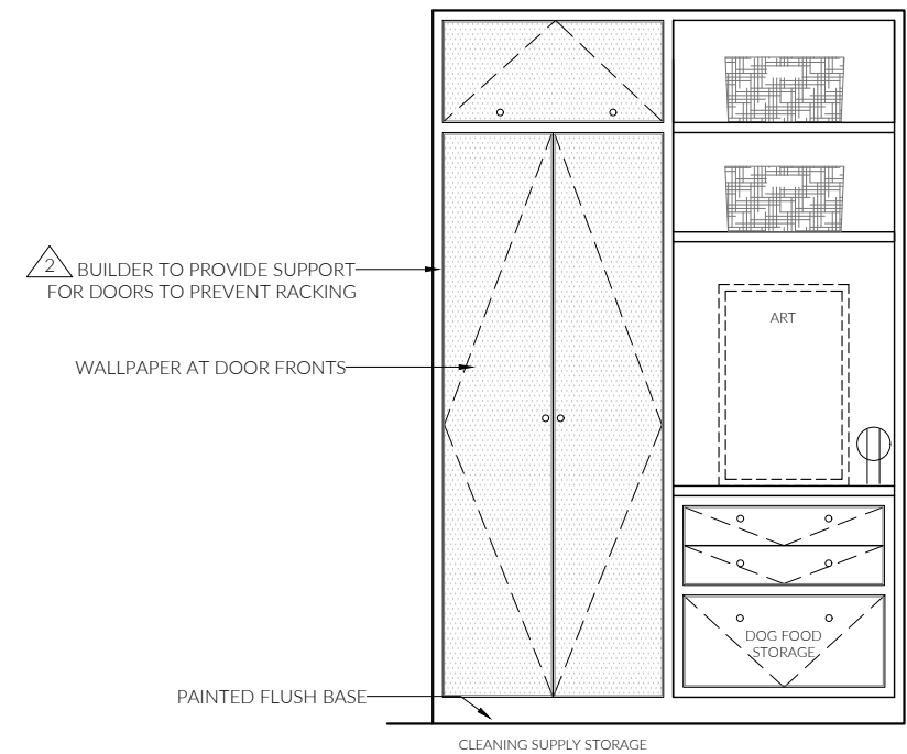
② MUDROOM - CLOSED
