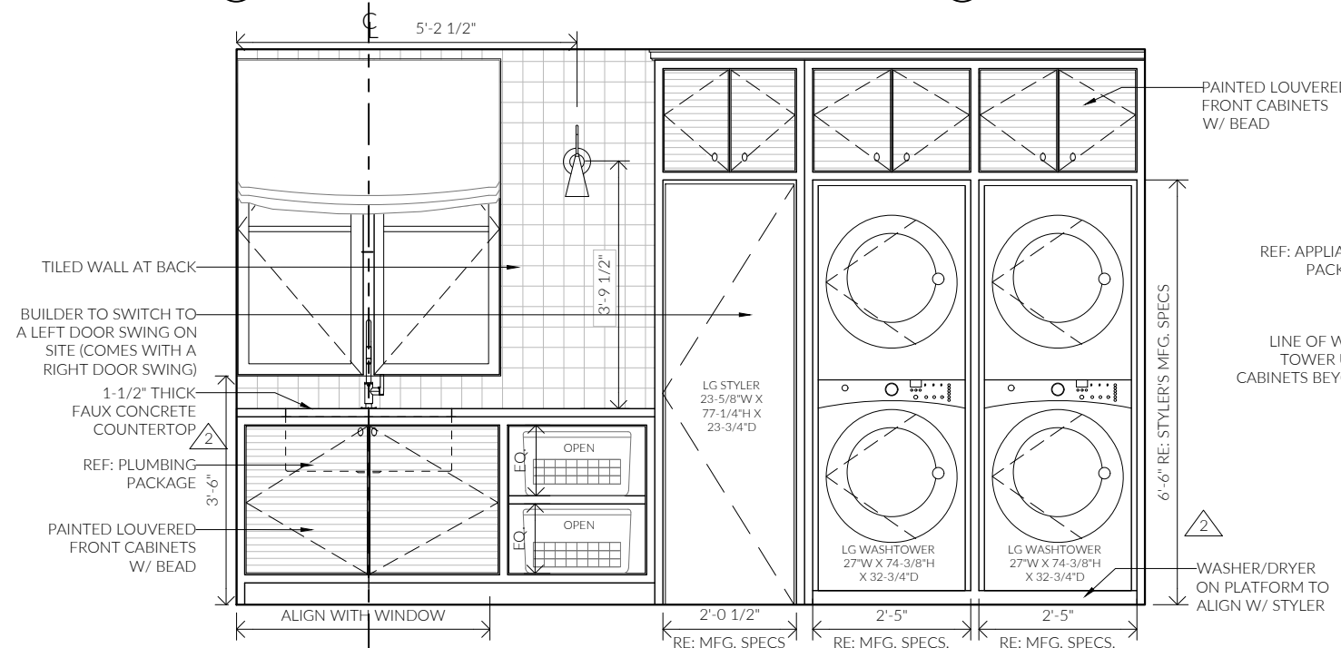
③ LAUNDRY ROOM
