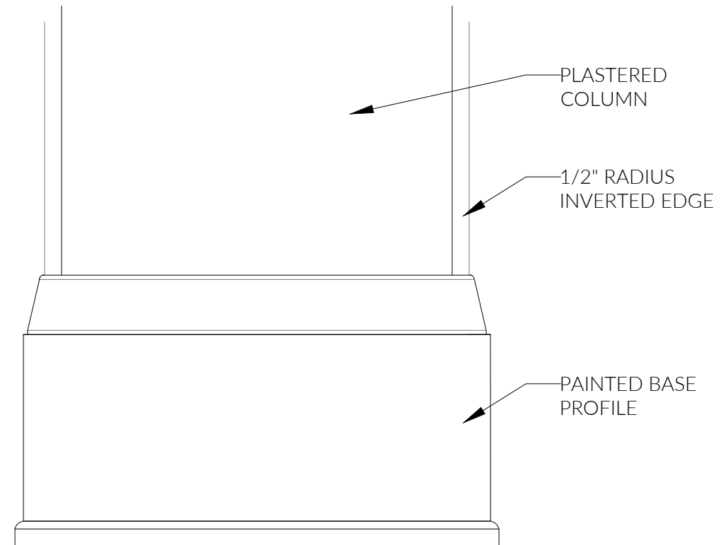
2.1 DETAIL - ELEVATION
