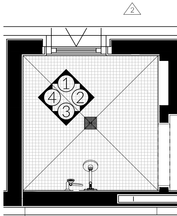
GUEST SHOWER ENLARGED PLAN SCALE: \frac{1}{2}" = 1'-0"
