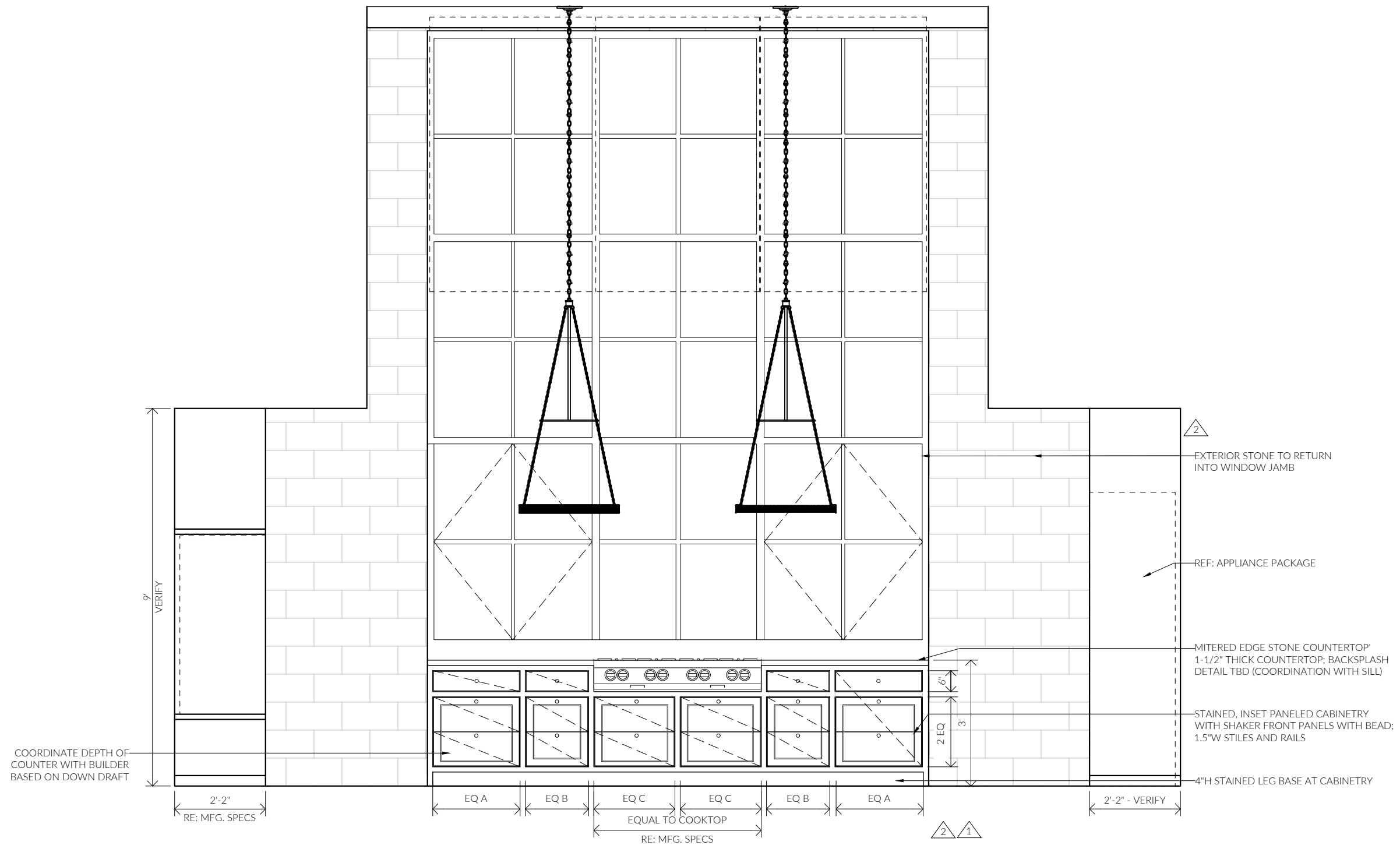
① KITCHEN SCALE: 3/8" = 1'
