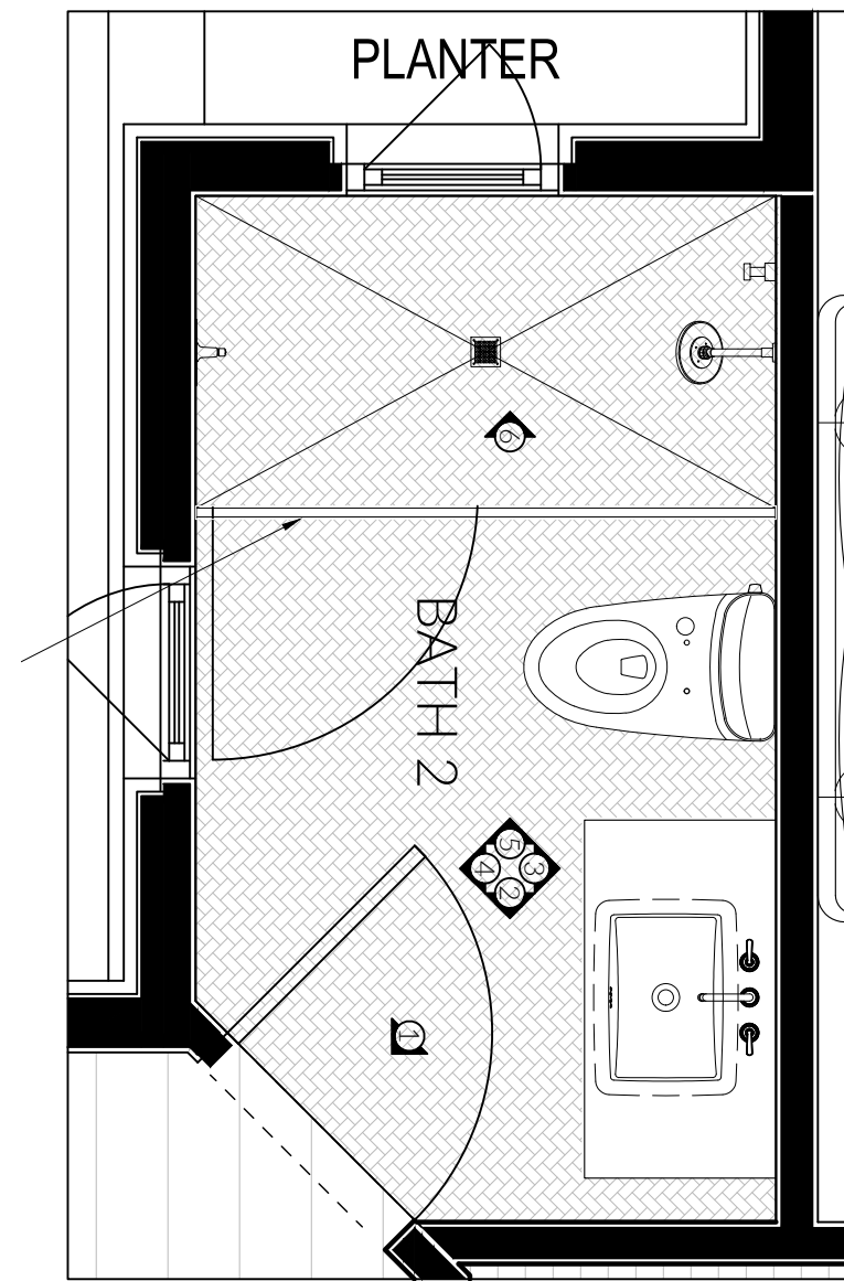
BATHROOM 2 ENLARGED PLAN SCALE: \frac{1}{2}" = 1'-0"
