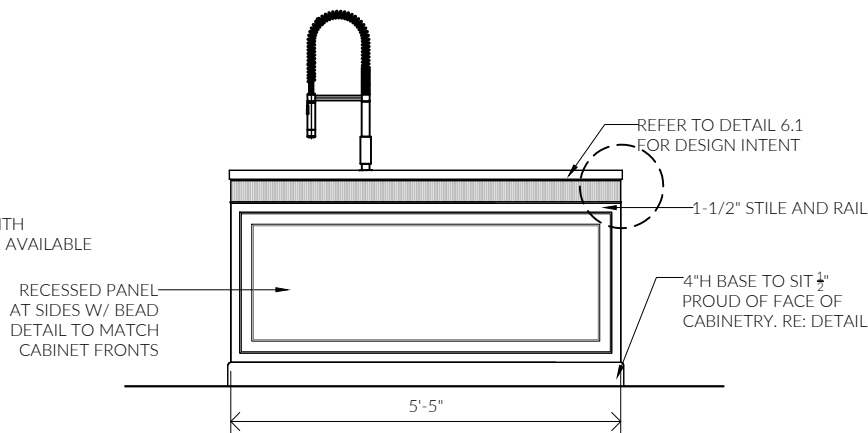
⑥ KITCHEN ISLAND SCALE: 3/8" = 1'0"
