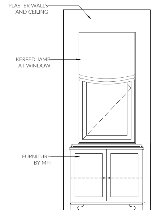
② POWDER ROOM 02 VEST.
