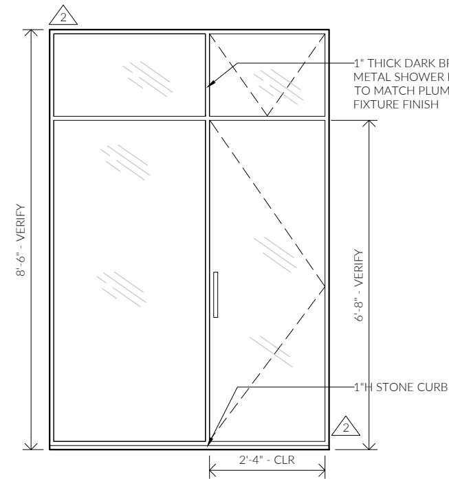
④ BATHROOM 3
