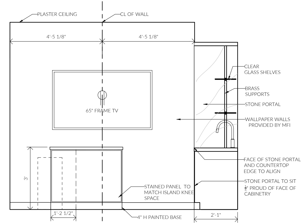
③ MAN CAVE BAR EAST
