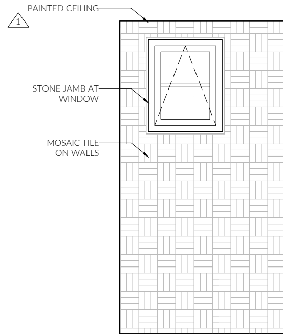
① BATH 4 SHOWER
