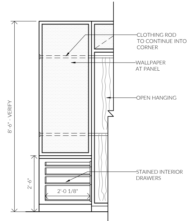
③ HER CLOSET
