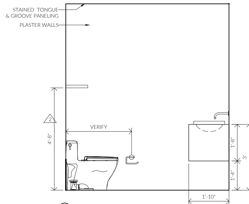
③ POOL POWDER ROOM
