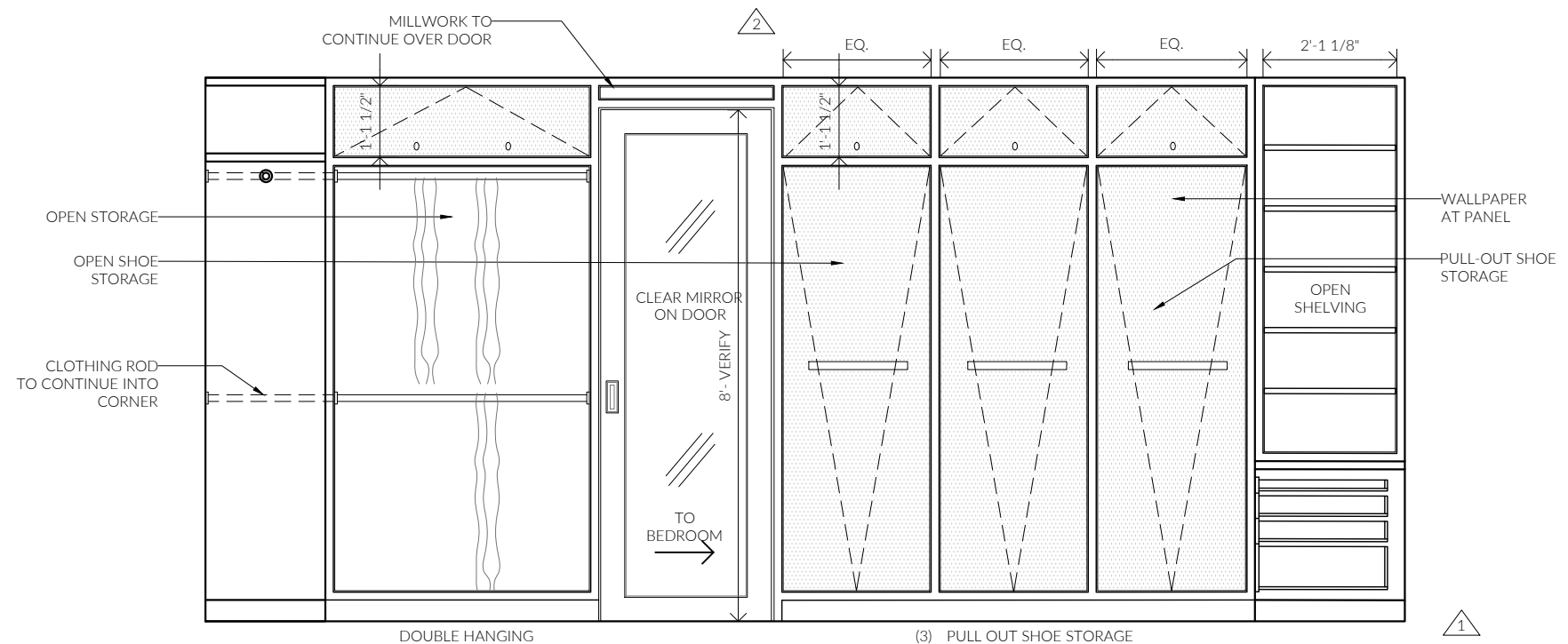
⑤ HER CLOSET
