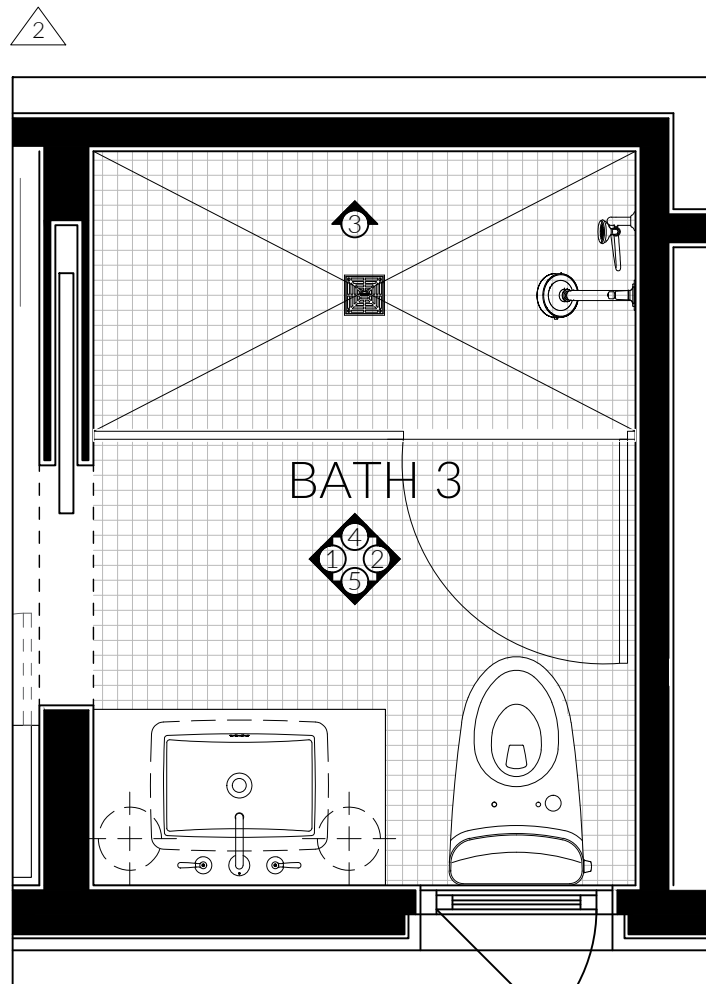
BATHROOM 3 ENLARGED PLAN SCALE: \frac{1}{2}" = 1'-0"
