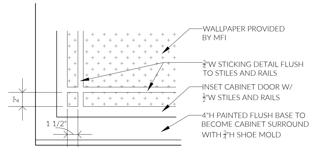
1.1 DETAIL
