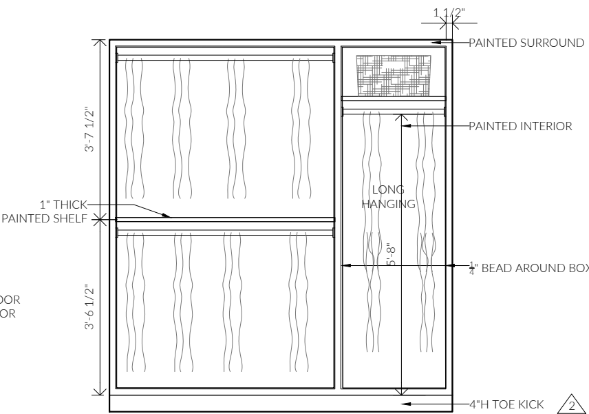
② BEDROOM 1 CLOSET
