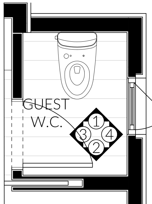
GUEST WC ENLARGED PLAN SCALE: \frac{1}{2}" = 1'-0"
