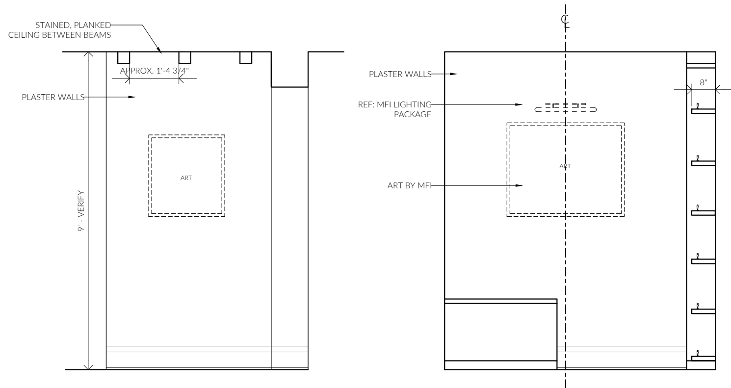
① BREAKFAST ROOM
