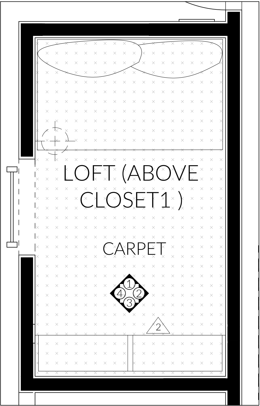
LOFT ENLARGED PLAN SCALE: 3/4" = 1'-0"
