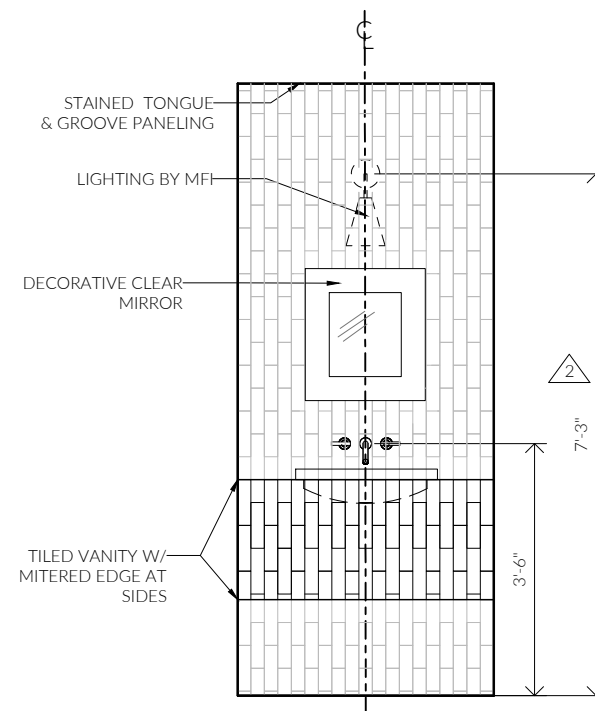
① POOL POWDER ROOM
