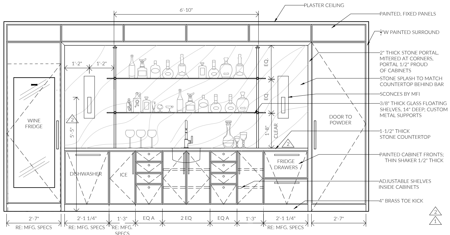
② MAN CAVE BAR NORTH
