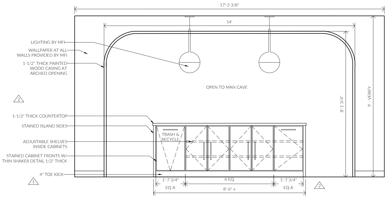
① MAN CAVE BAR NORTH
