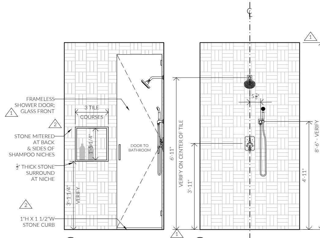
② BATH 4 SHOWER
