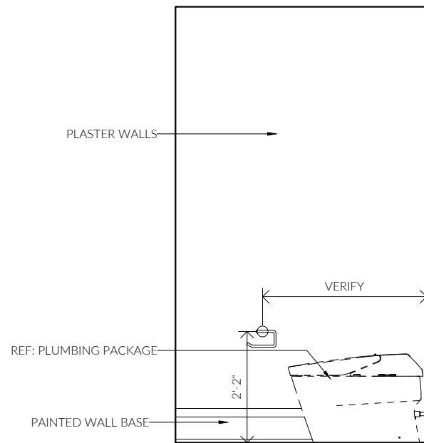
① MASTER BATH W.C.
