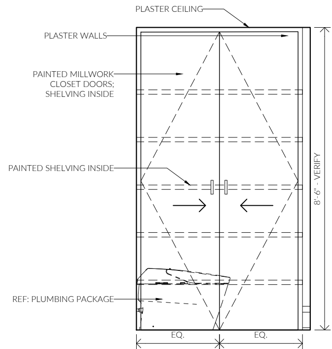
② MASTER BATH W.C.
