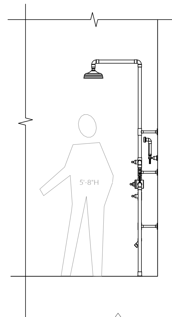
② OUTDOOR SHOWER
