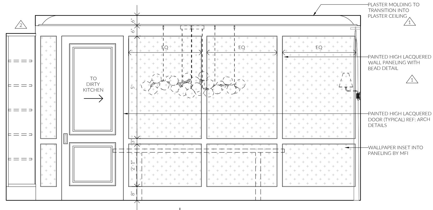
② DINING ROOM
