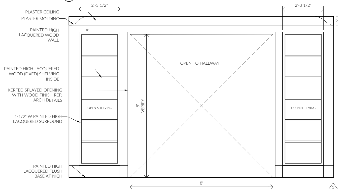
③ DINING ROOM
