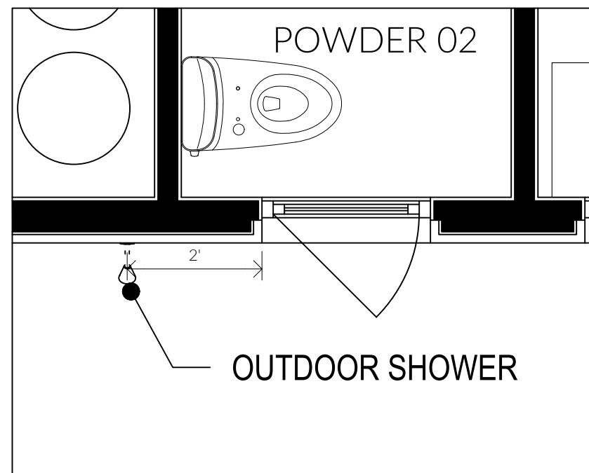
OUTDOOR SHOWER ENLARGED PLAN SCALE: 1/2" = 1'-0"
