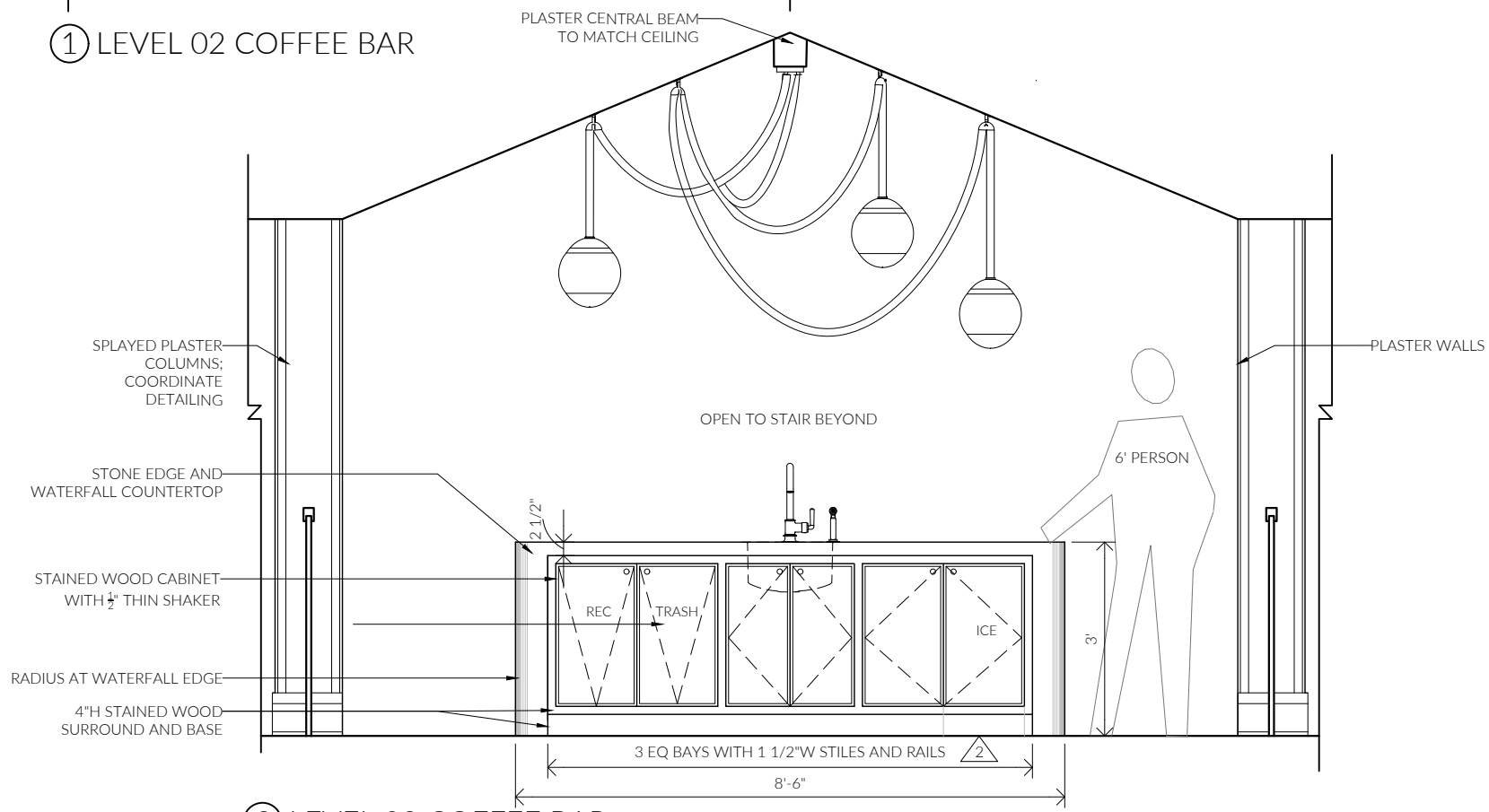
② LEVEL 02 COFFEE BAR
