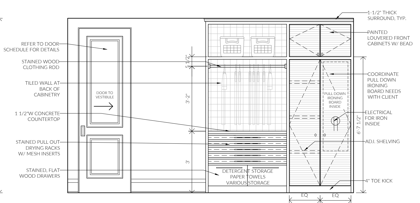
② LAUNDRY ROOM
