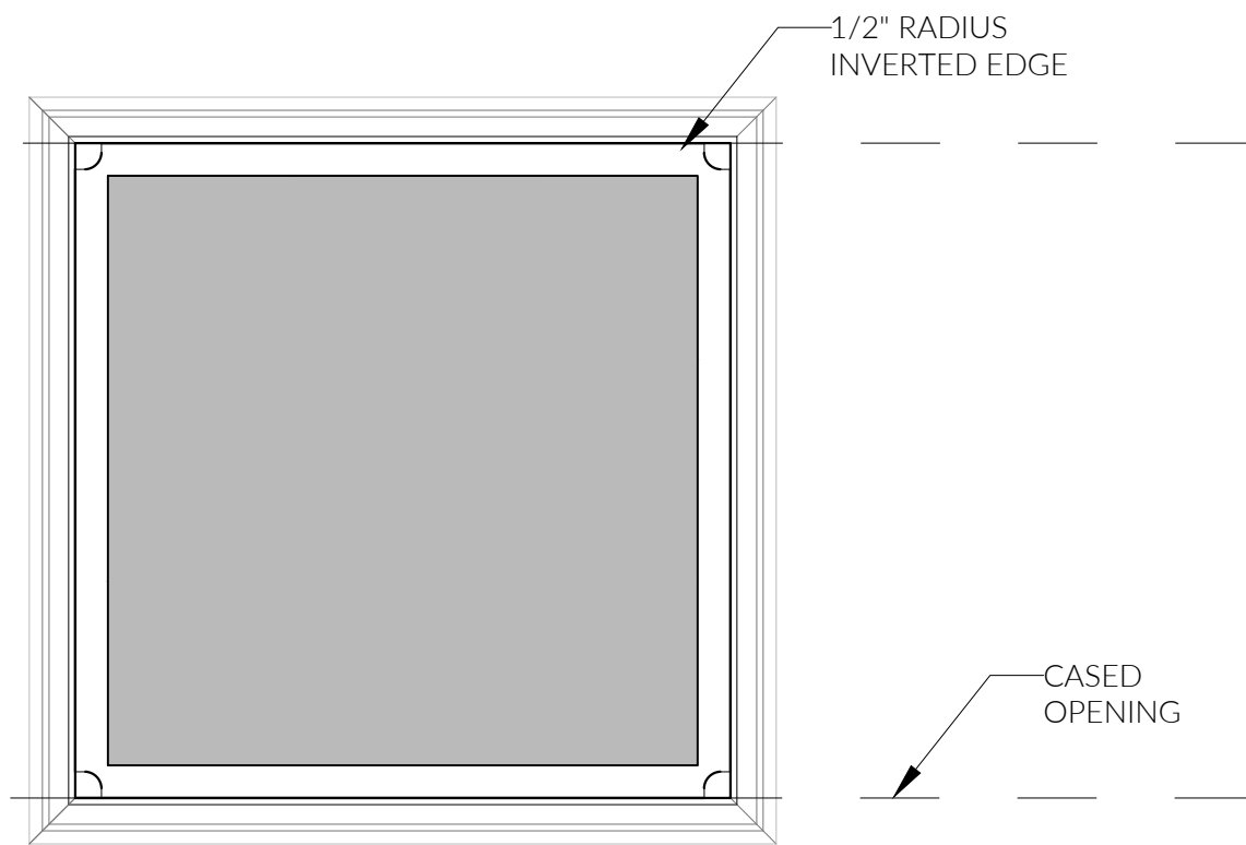
2.1 DETAIL - PLAN
