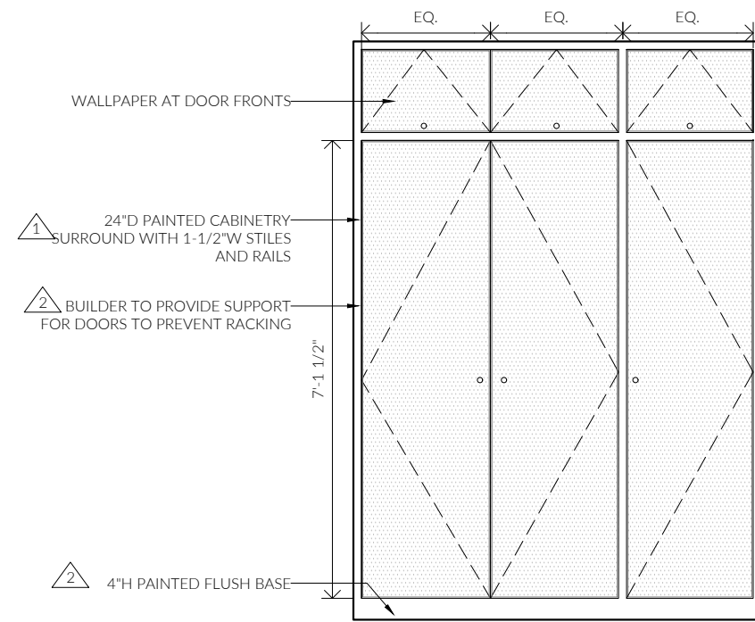
① MUDROOM - CLOSED
