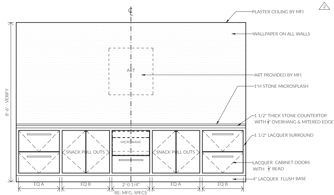
① THEATER SNACK ROOM
