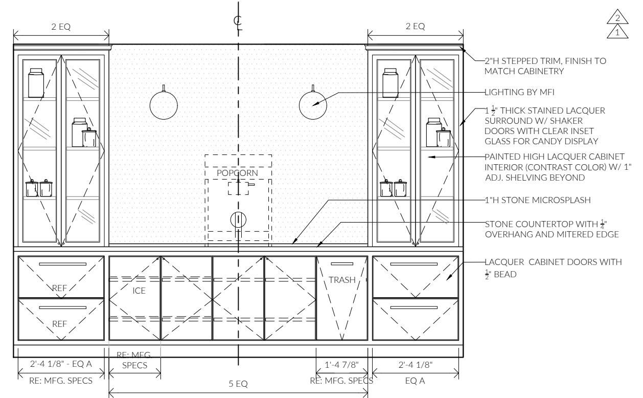
② THEATER SNACK ROOM
