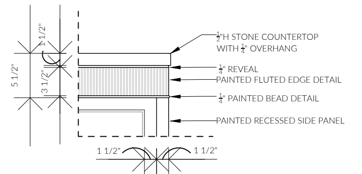
⑥.1 DETAIL SCALE= 1"-1'0"
