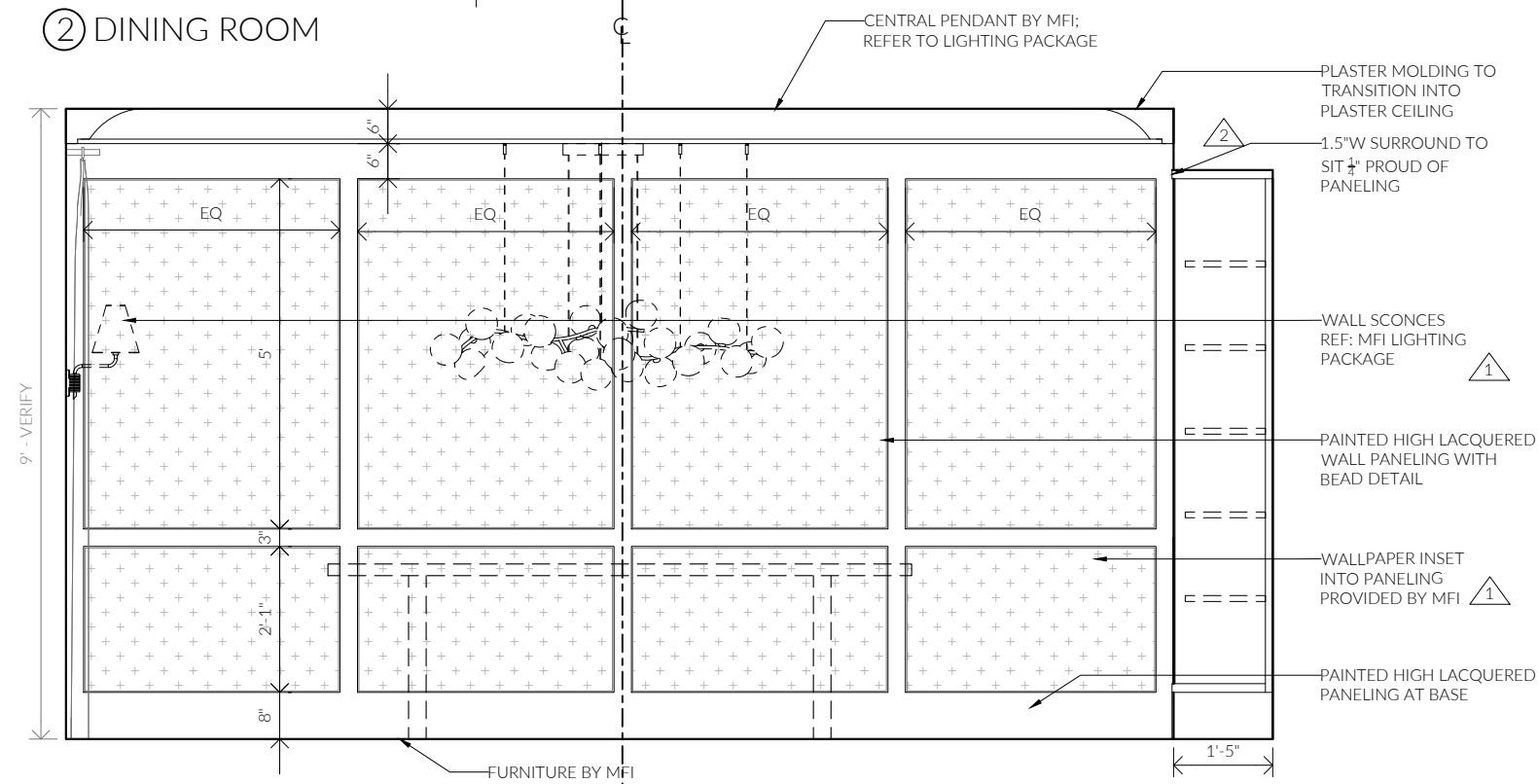
④ DINING ROOM
