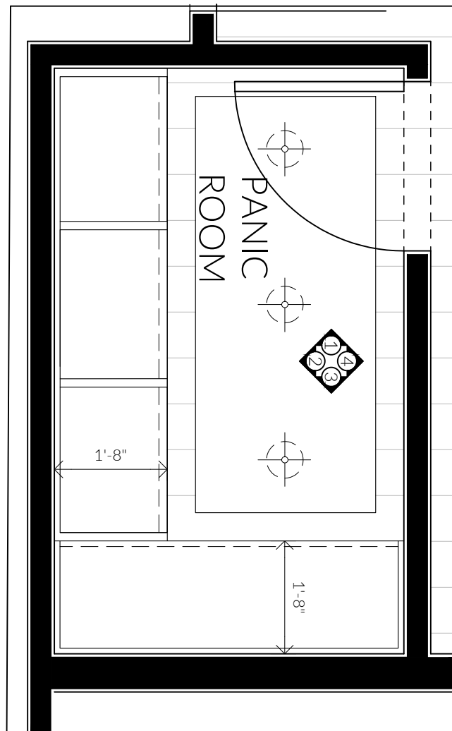
PANIC ROOM ENLARGED PLAN SCALE: \frac{1}{2} " = 1'-0"
