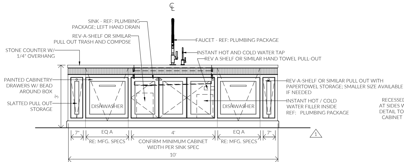
④ KITCHEN ISLAND SCALE: 3/8" = 1'0"
