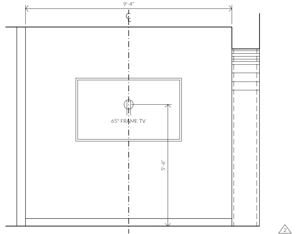
④ MAN CAVE BAR WEST
