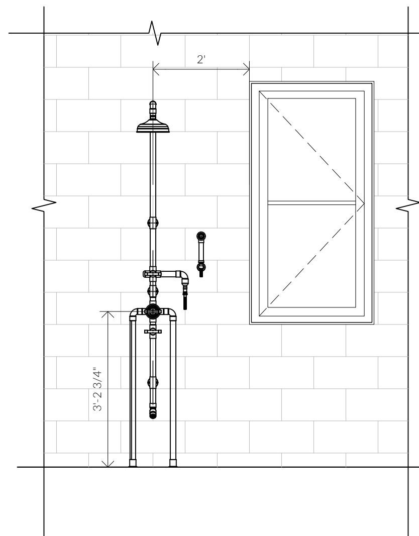
① OUTDOOR SHOWER
