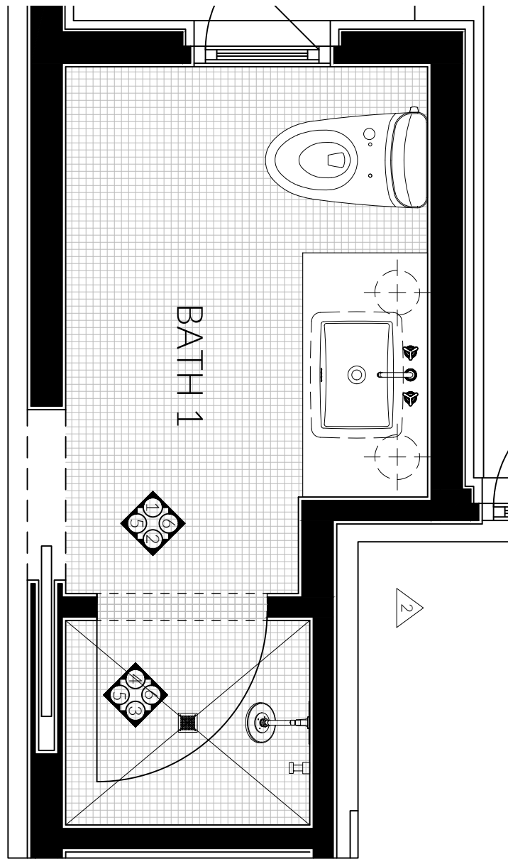
BATHROOM 01 ENLARGED PLAN SCALE: \frac{1}{2}" = 1'-0"
