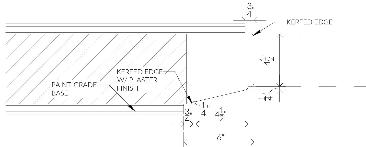
1.3 DETAIL - PLAN
