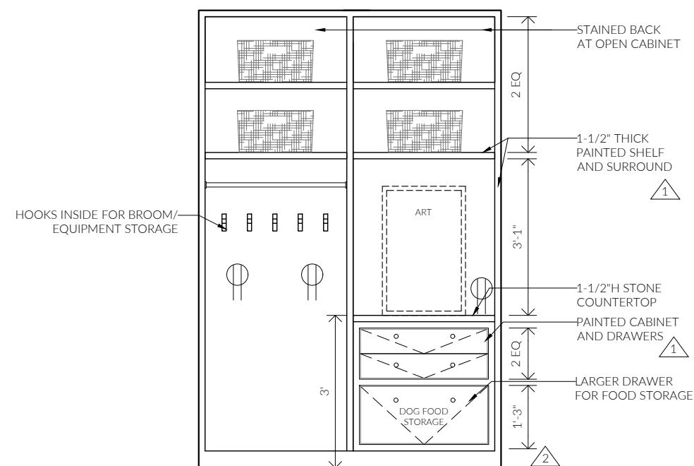
② MUDROOM - OPEN
