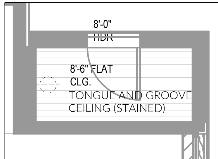
ENLARGED RCP
